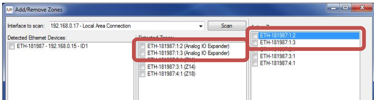
Figure 49 – Adding an Ethernet IO Board with inputs configured as analog inputs
