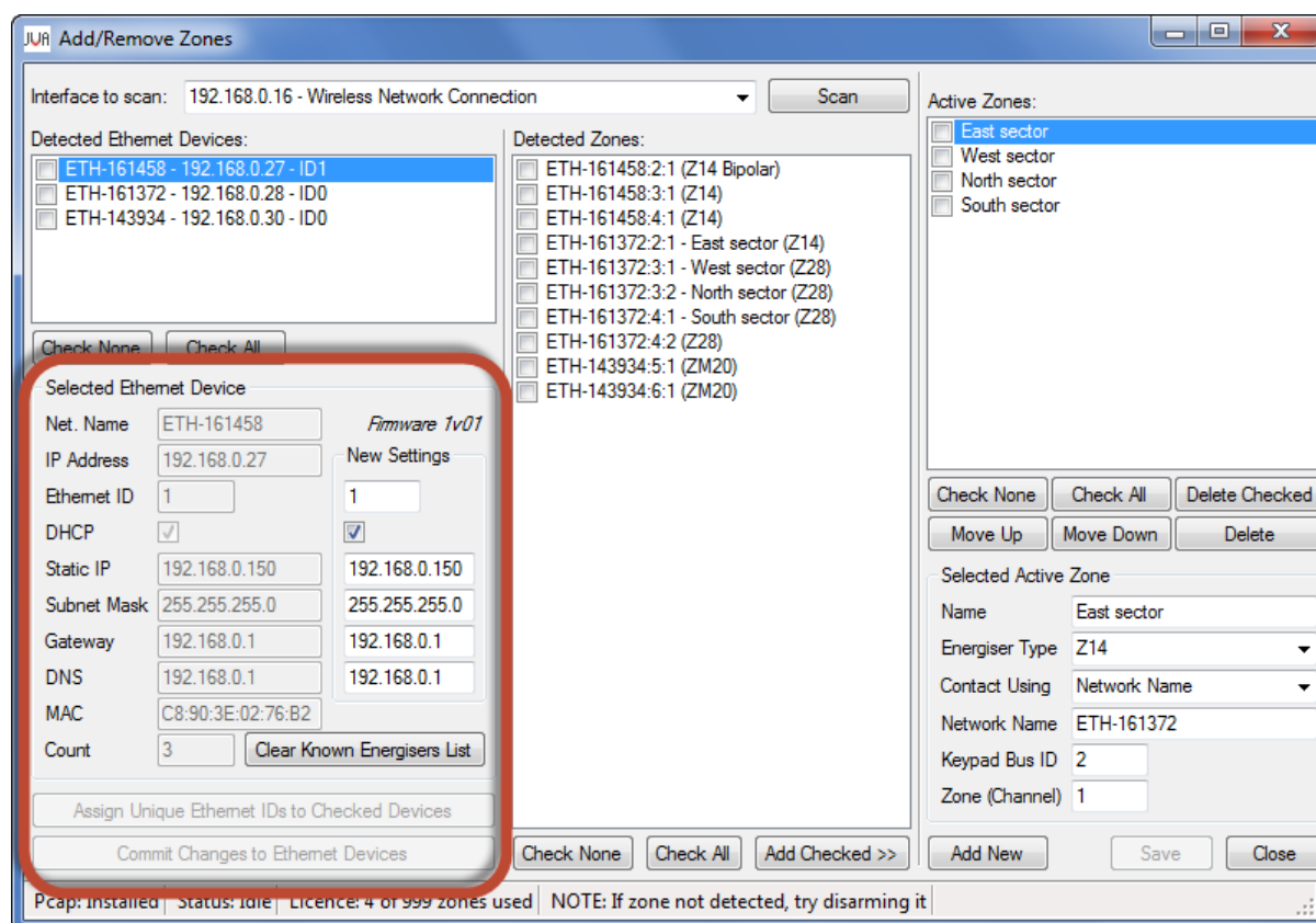
Figure 38 - Configuration Settings for a PAE212 Ethernet Adapter Device
