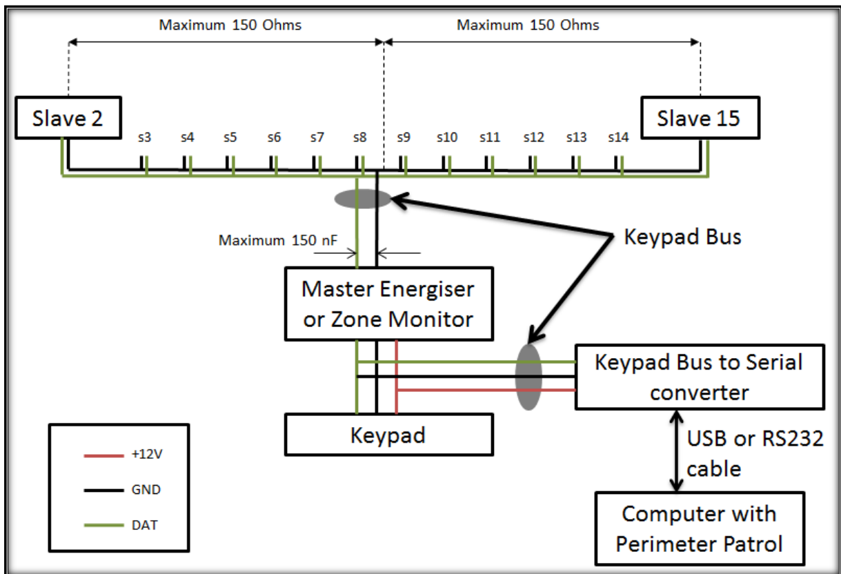
Figure 5 – Connecting a PAE051/PAE223 to JVA Perimeter Patrol via RS232 or USB cable
