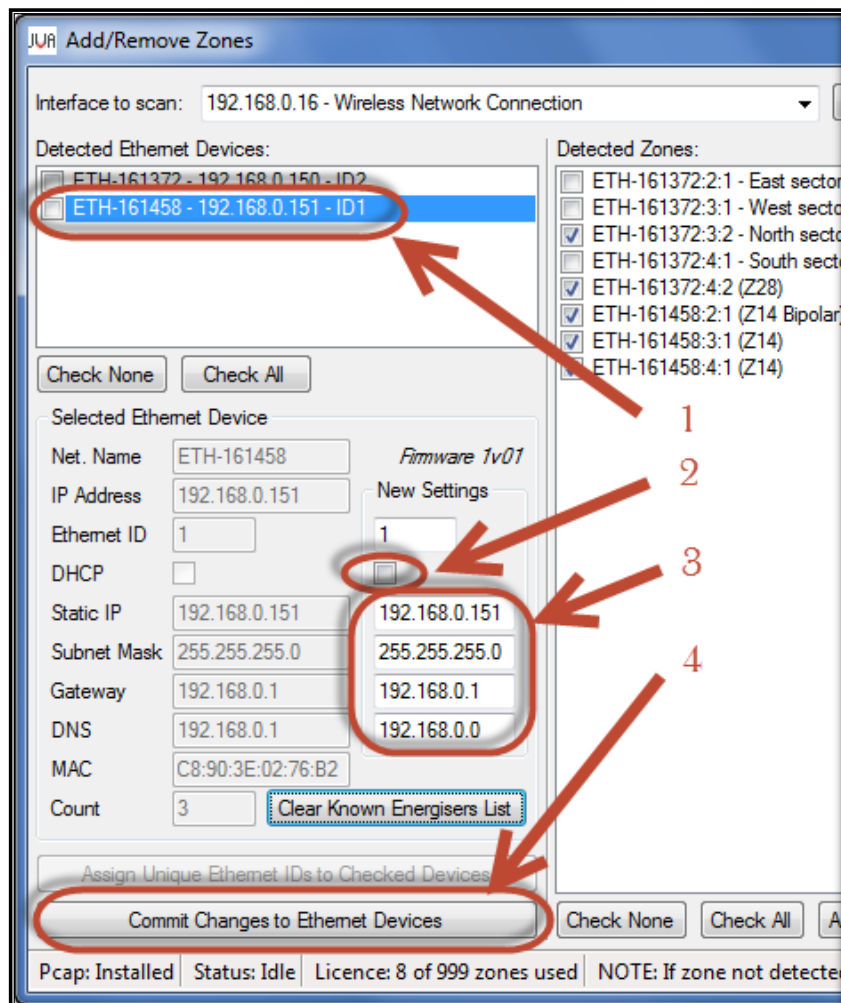
Figure 39 - Configuring each PAE212 Ethernet Adapter Device to use Static IP Address. Note that DHCP is UNSELECTED.
